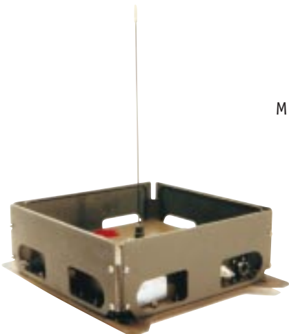
MA1310 DF Antenna Frequency Range: 150 to 1300 MHz
