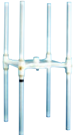
AA381EW DF Antenna Frequency Range: 80 to 250 MHz
